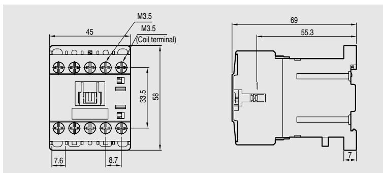
GMR-4MD
